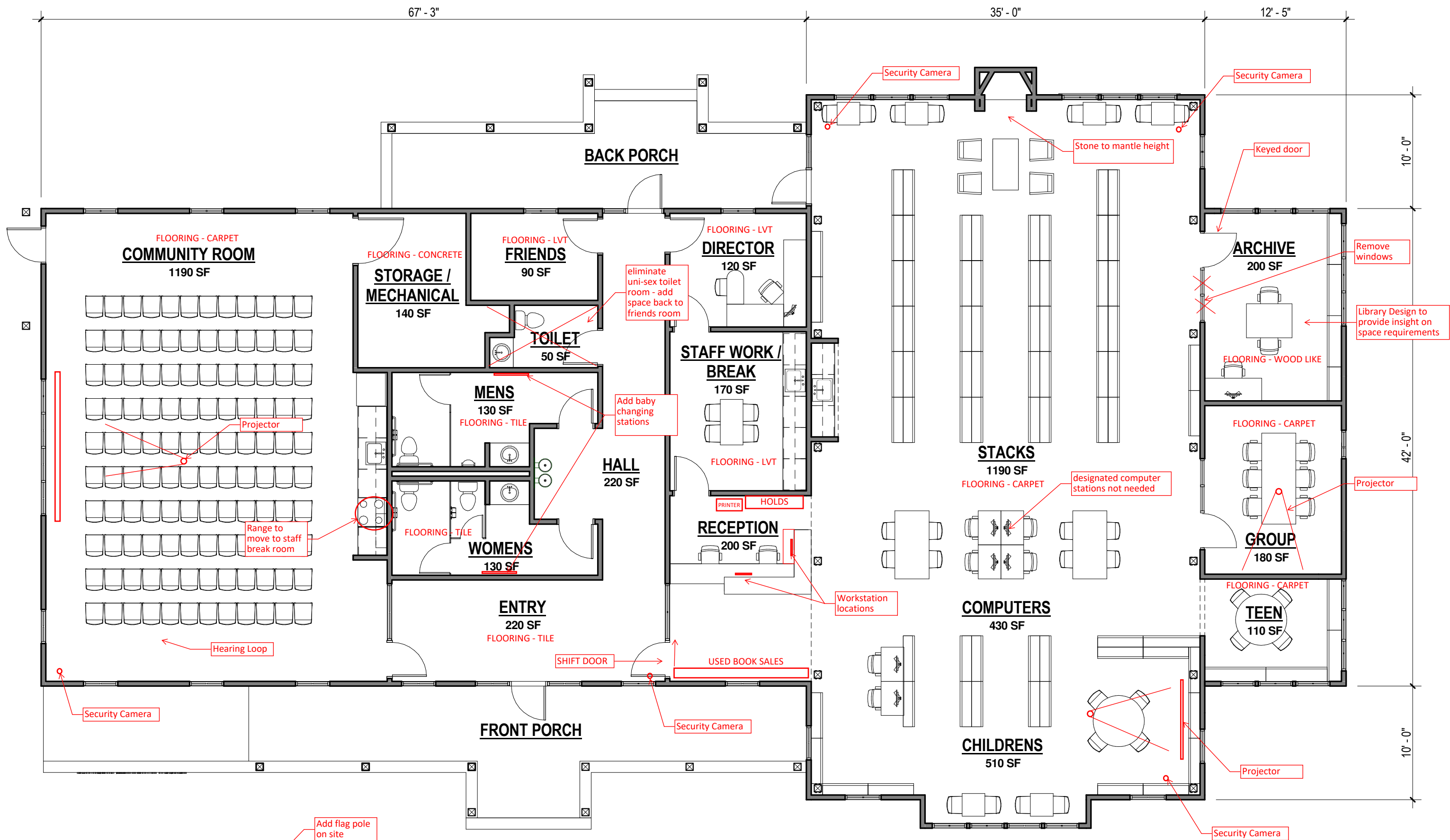
Floor Plan - 02-16-18
